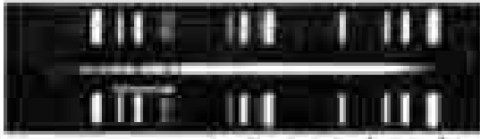
URSA MAJOR
