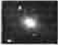
URSA MAJOR
