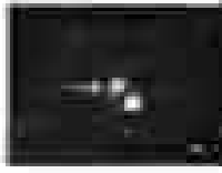
BOOTES
