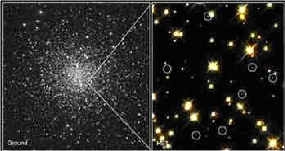
White Dwarf Stars in M4 HST - WFPC2 PRC95-32 - ST ScI OPO - August 26, 1995 - H. Bond (ST ScI), NASA
