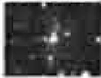
HYDRA
