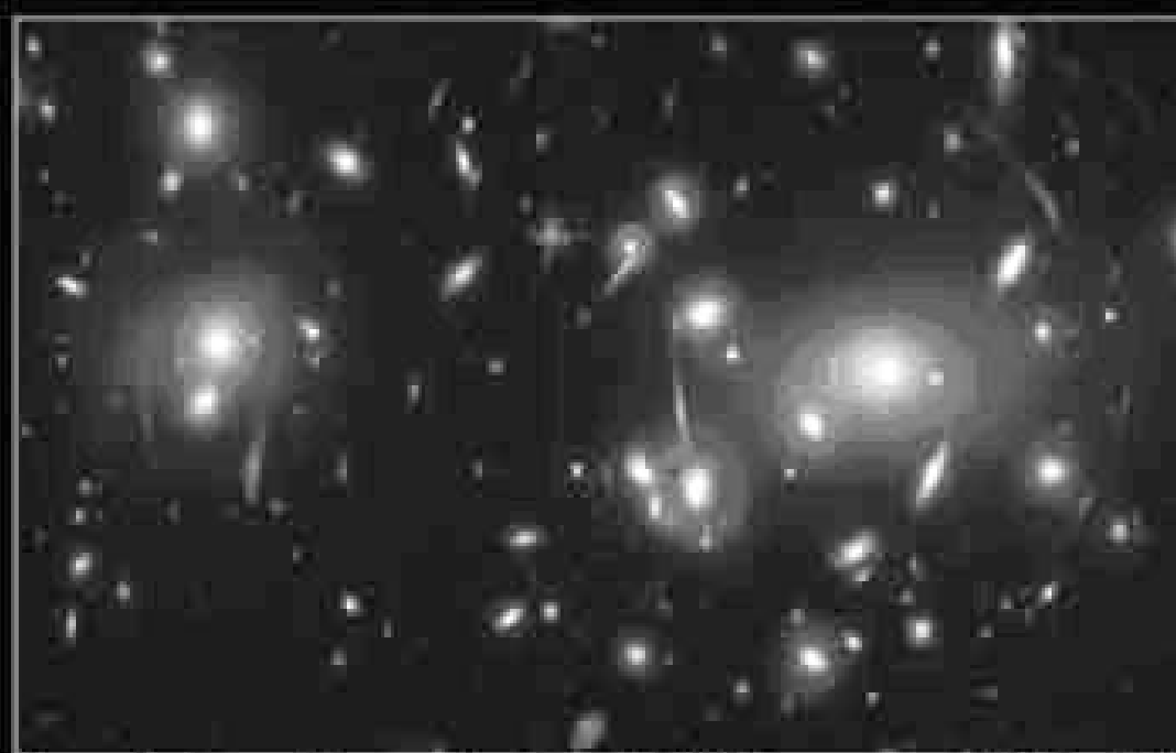
Gravitational Lens in Abell 2218
